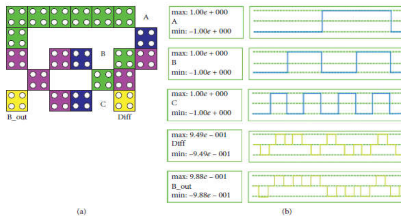
Figure 3: (a) layout of the proposed full adder and (b) its simulation results.
