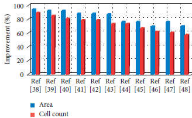
Figure 4: Improvements of proposed adder over others.
