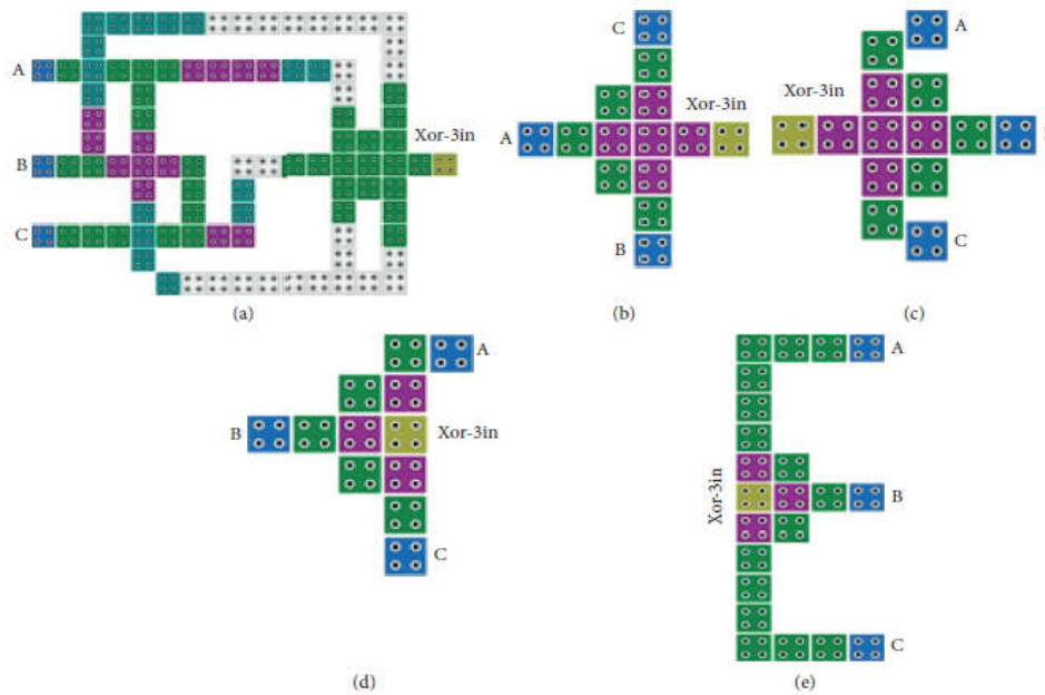
Figure 2: Previous three-input XOR gate based on QCA technology. (a) [20], (b) [21], (c) [22], (d) [23], and (e) [24].
