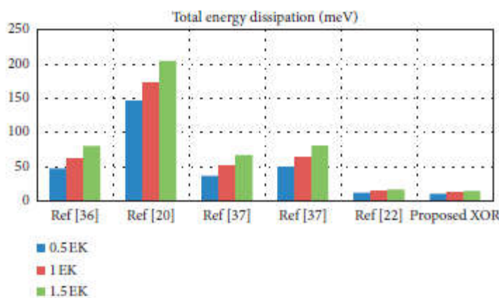
Figure 5: total energy dissipation of the adders at three different tunneling energy levels.
