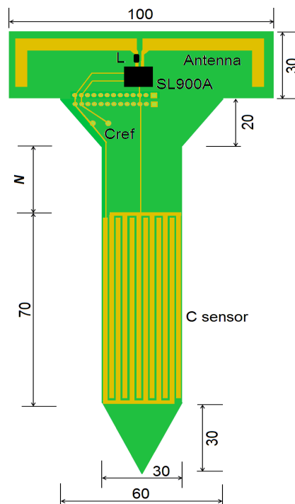
Figure 7. Design of the Soil Stick Sensor using UHF RFID chip (SL900A) and an interdigital capacitive humidity sensor ( C_{sensor} ). A neck of N = 30 mm was defined. The arrow shape allows the tag to be stuck into soil. The whole sensor area must be buried. All dimensions are in millimeter (mm).
